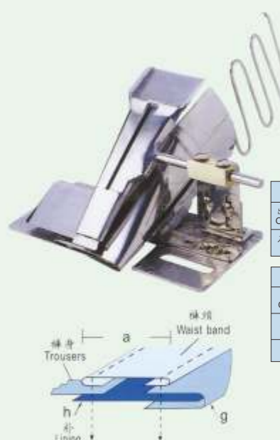
JZ-15541 F325 西裤裤头拉筒 Casual Trousers Waist Band Folder
