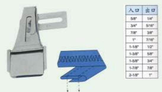
JZ-15507 F340 耳仔筒 Belt Loop Folder
