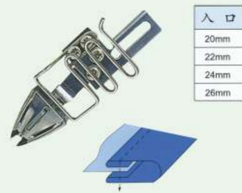
JZ-15517 祖奇包缝车包边筒 Edge Binder for Pegasus Overlock Machine
